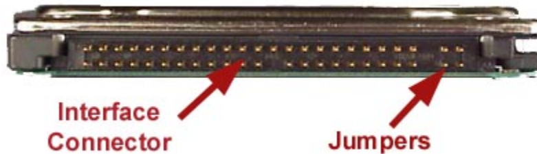
Figure 1.MK3019GAX HDD Rear View - Connectors
